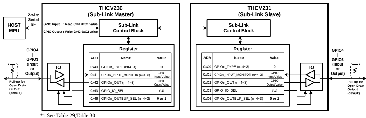
Figure 14. Programmable GPIO
