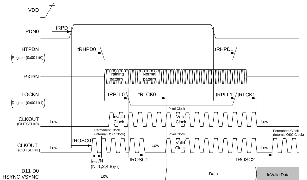
Figure 25. THCV231 Lock/Unlock Sequence
