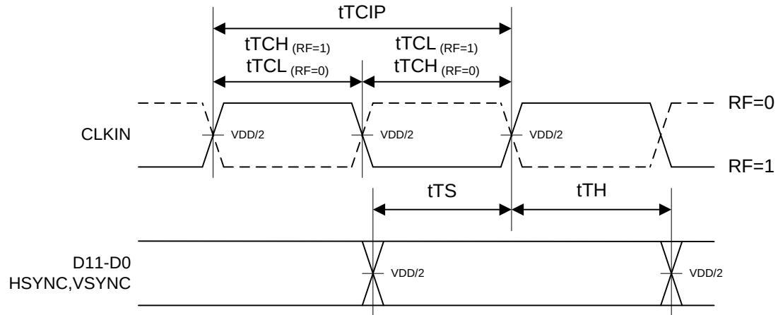
Figure 17. LVC MOS Input Switching Timing Diagrams
