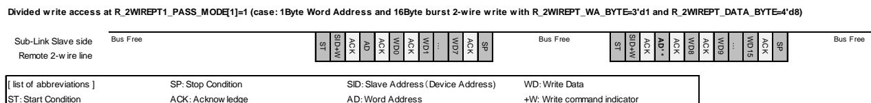
Figure 12. 2-wire Pass Through mode1 Sub-Link Slave command Divided scheme
