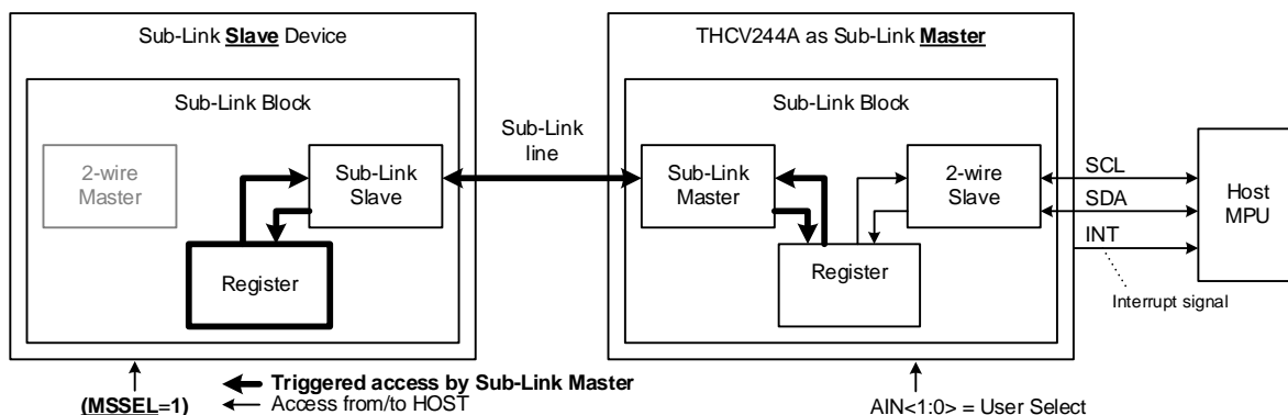
Figure 9. Host MPU to Sub-Link Slave Register via THCV244A access configuration
