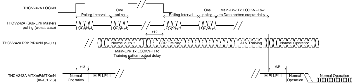
Figure 18. Re-Lock Sequence
