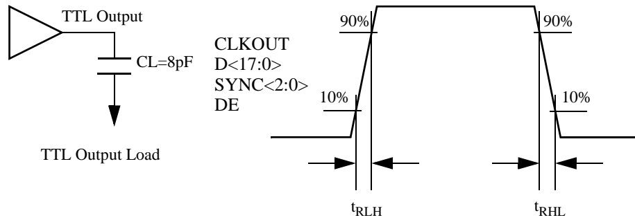
Fig. 4 CMOS/TTL Outputs Load and Transition Time
