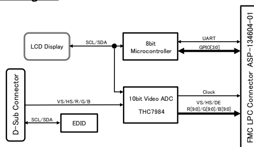
Block Diagram
